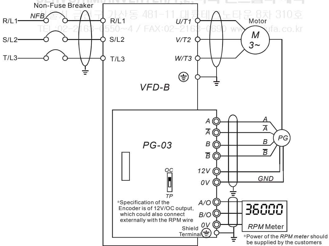
Connection between PG-03 and the Encoder
