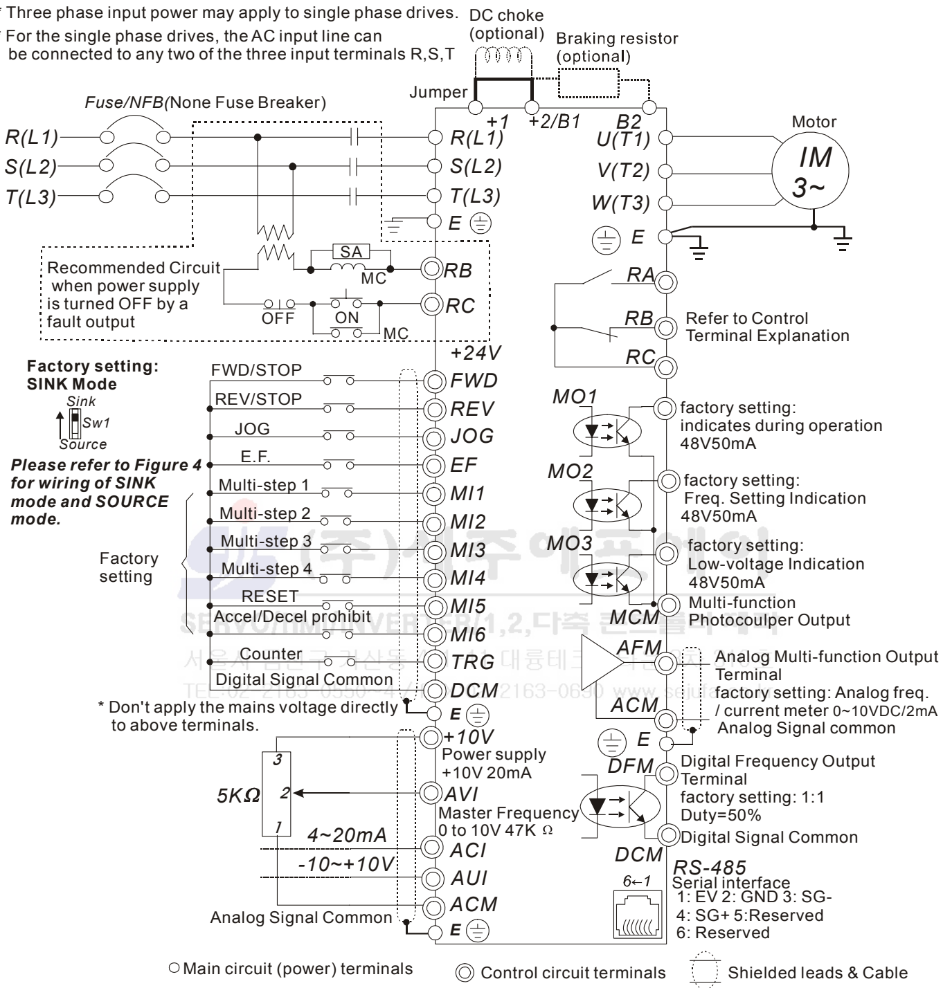
Figure 1 for models of VFD-B Series VFD007B21A/23A/43A/53A, VFD015B21A/21B/23A/23B/43A/53A, VFD022B23B/43B/53A
