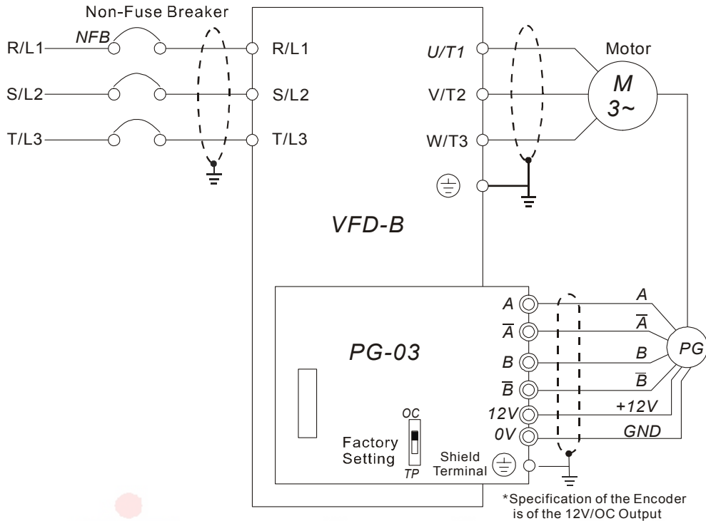
Connection between PG-03 and the Encoder
